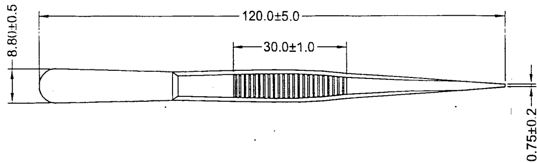
SIDE ELEVATION
